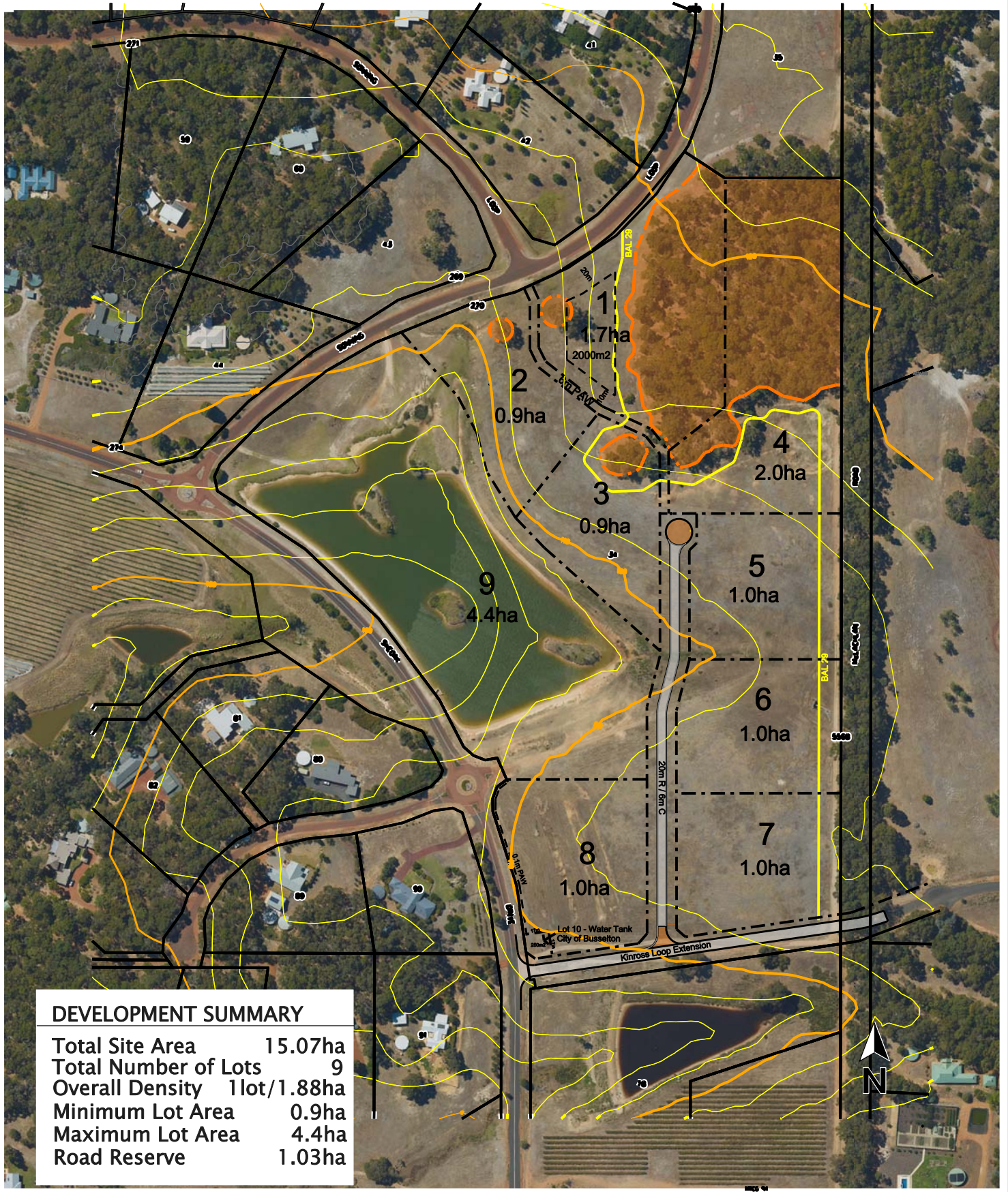
STRUCTURE PLAN : LOT 34 SHEOAK DVE, YALLINGUP FIGURE 2
